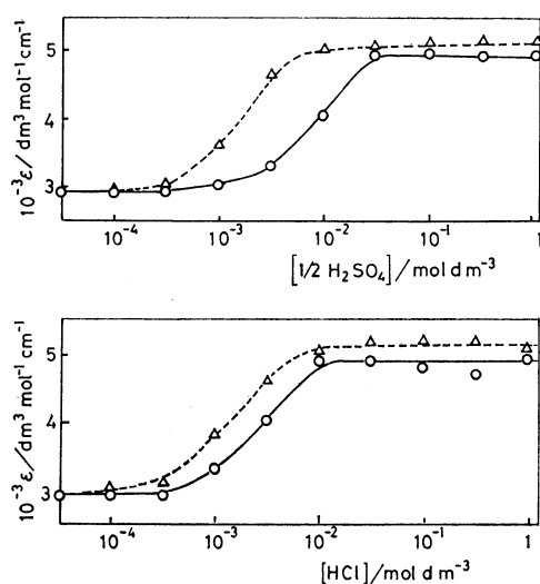
Fig. 3. Relation between the molar absorption coefficients of 1 and the concentration of mineral acids. --- \triangle ---: [\mathbf{1}] = 10^{-3} \text{ mol dm}^{-3} , --- \circ ---: [\mathbf{1}] = 3 \times 10^{-3} \text{ mol dm}^{-3} .
